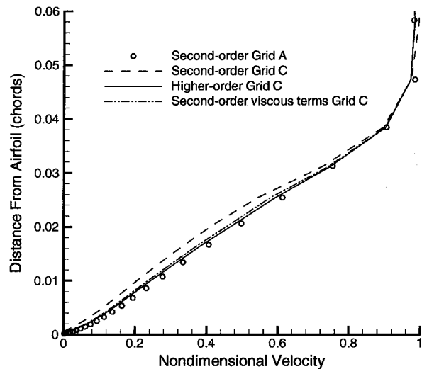
Fig. 10 Boundary-layer velocity profiles on the upper surface at 95% chord; RAE 2822 airfoil, M_\infty = 0.754 , \alpha = 2.57 deg.
