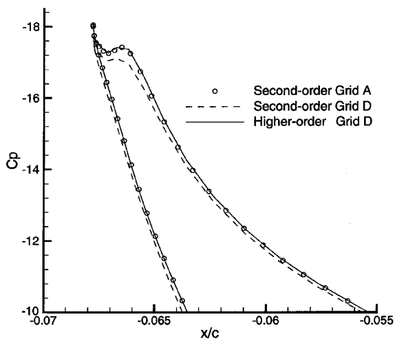
Fig. 13 Pressure distribution on upper surface of slat.
