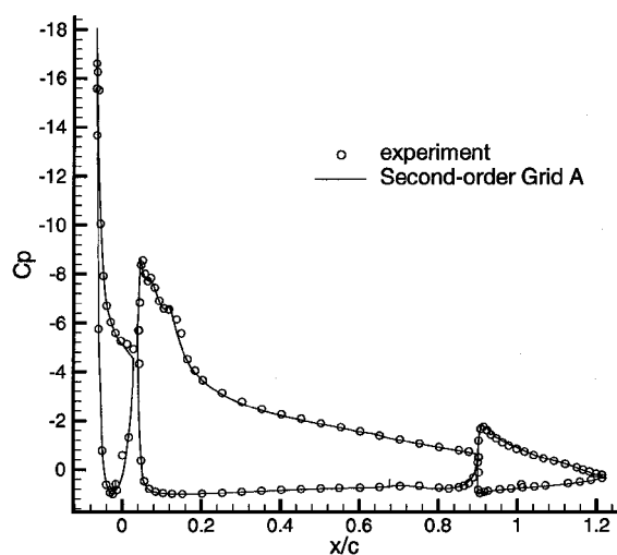
Fig. 12 Pressure distribution for the three-element geometry.
