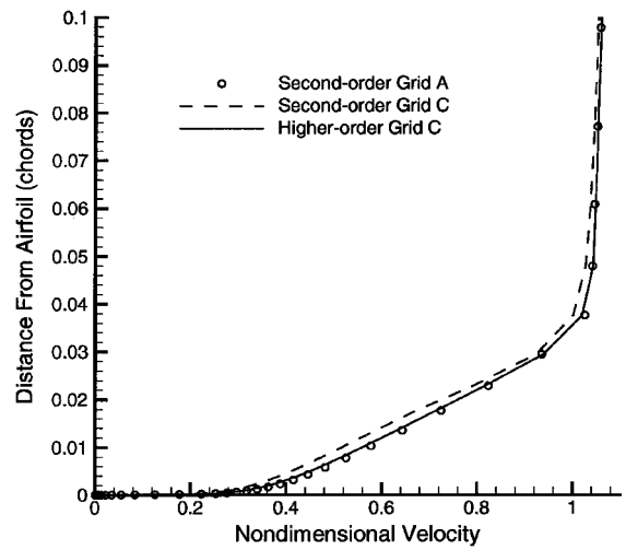
Fig. 6 Boundary-layer velocity profiles on the upper surface at 85% chord: case 1.
