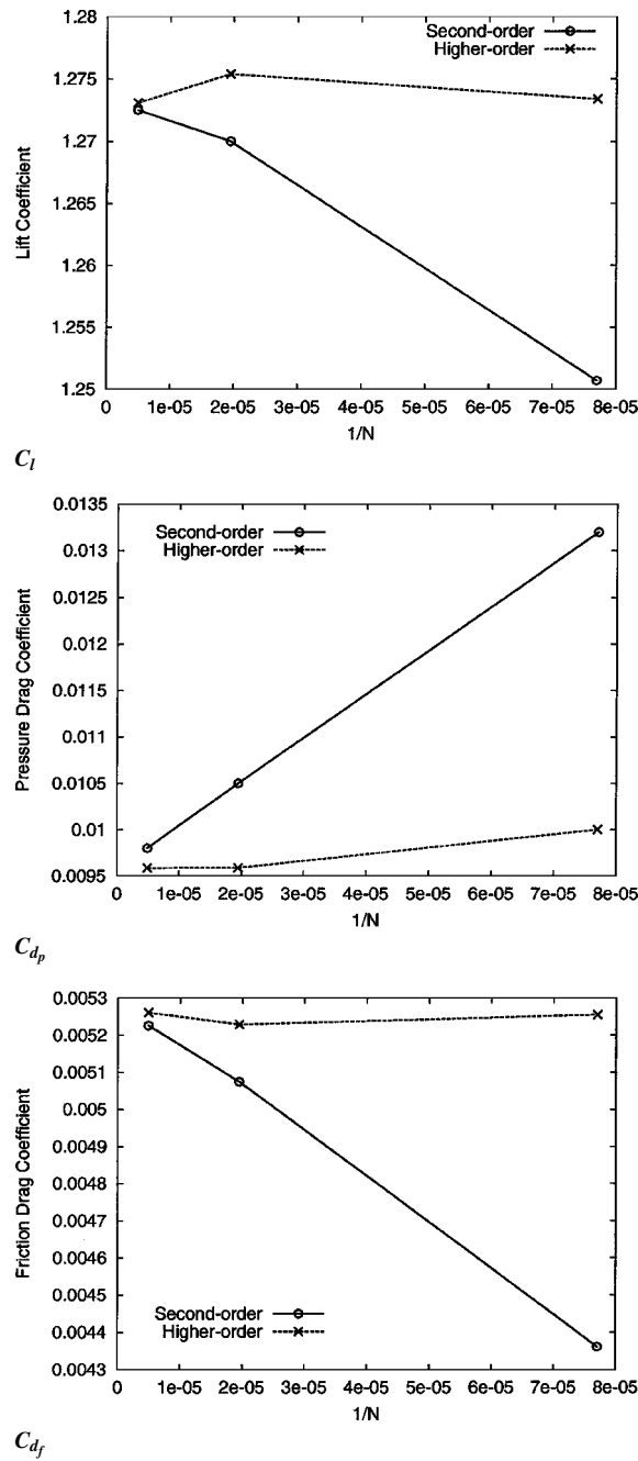
Fig. 5 Grid convergence for case 1.
