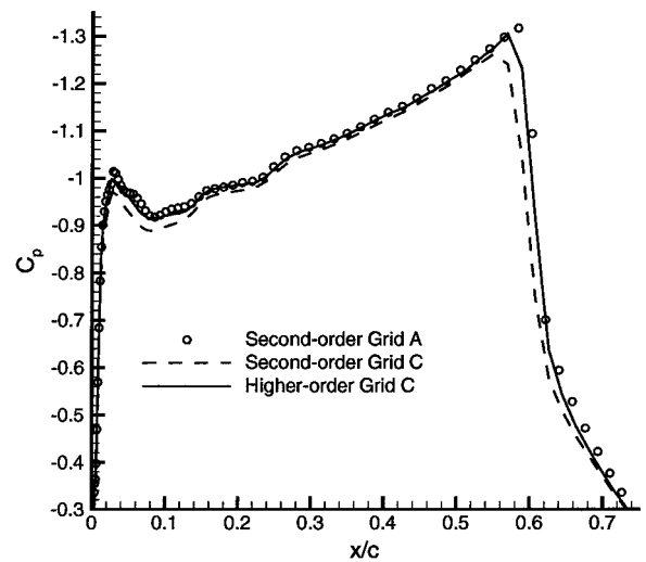
Fig. 9 Pressure coefficient on the upper surface; RAE 2822 airfoil, M_\infty = 0.754 , \alpha = 2.57 deg.
