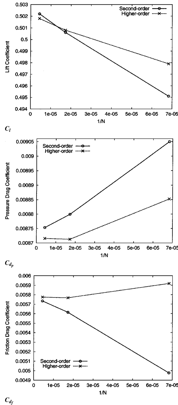
Fig. 7 Grid convergence for case 2.
