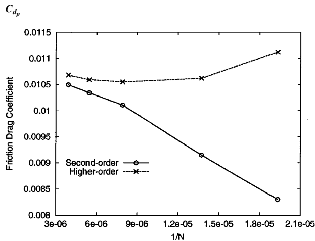
Fig. 11 Grid convergence for case 4.
